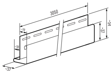
SV(P) 18 Conector
