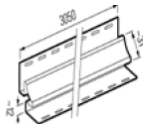
SV(P) 13 Esquina interior
