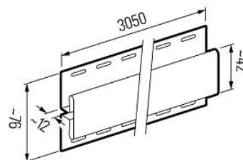
SV(P) 18 Conector
