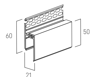
FS-11.5 Bottom ventilation trim
