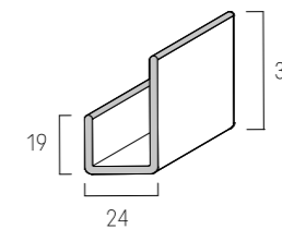
FS-251 Universal trim U
