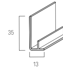
FS-251 Universal trim U
