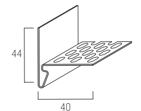
FS-11.5 Bottom ventilation trim
